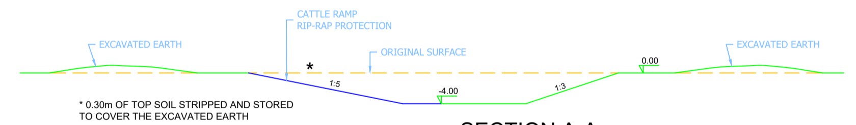
SECTION A-A SCALE 1:500
