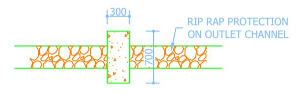
SECTION H-H SCALE 1:50
