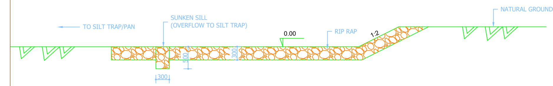
CROSS SECTION A-A SCALE 1:50
