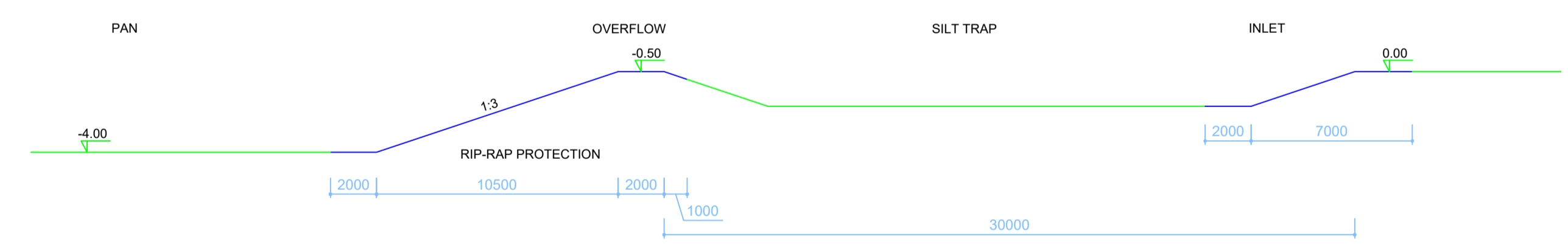
SILT TRAP DETAIL (B-B) SCALE 1:200
