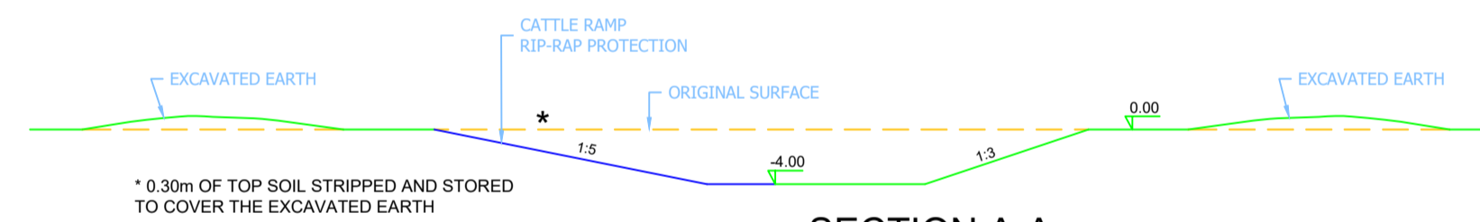
SECTION A-A SCALE 1:500
