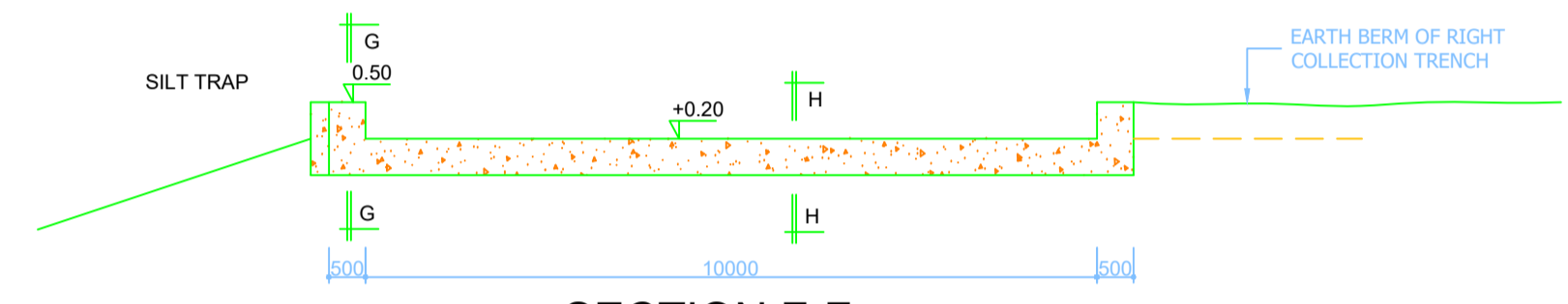
SECTION F-F OVERFLOW TO OUTLET CHANNEL SCALE 1:100
