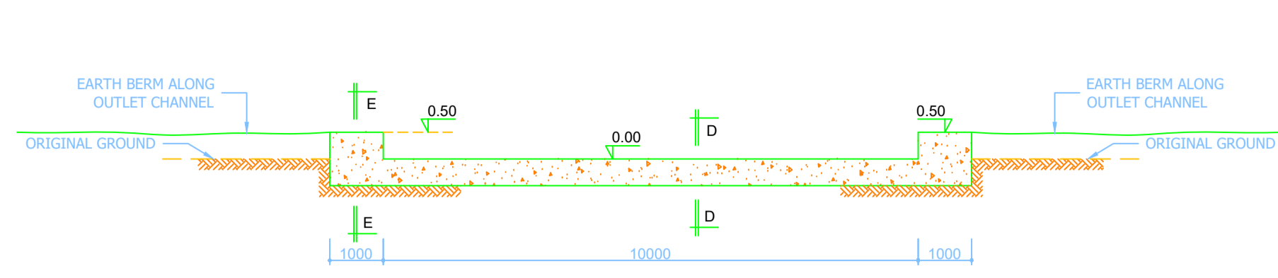
SECTION C-C INLET SILL TO SILT-TRAP SCALE 1:100
