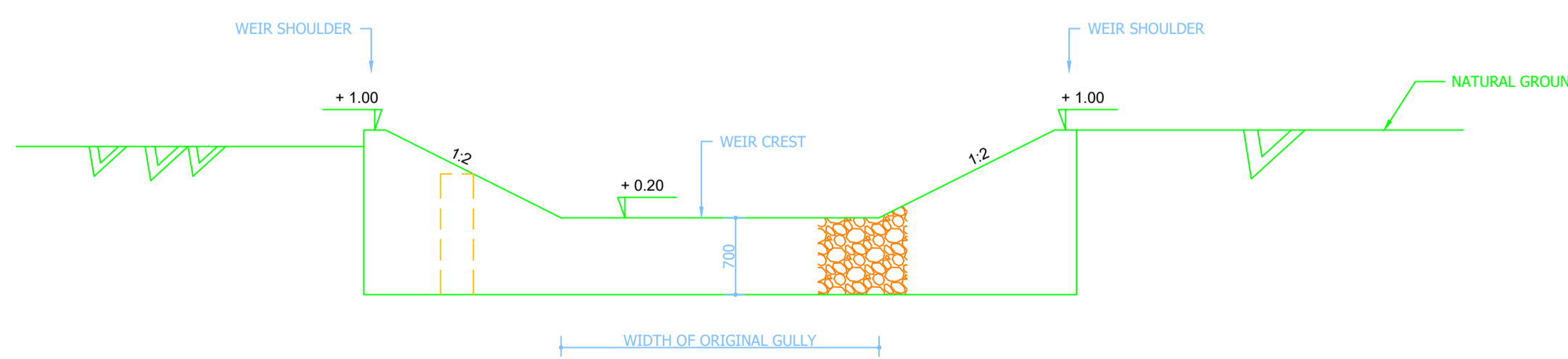
CROSS SECTION B-B SCALE 1:50
