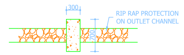
SECTION H-H SCALE 1:50
