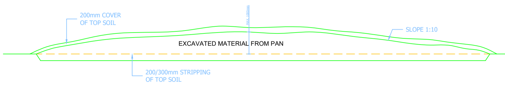
TYPICAL SECTION OF DISPOSED MATERIAL SCALE 1:100
