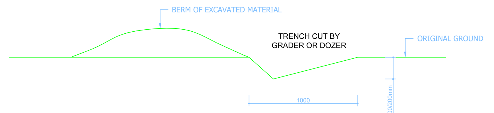
TYPICAL SECTION OF COLLECTION TRENCH SCALE 1:20
