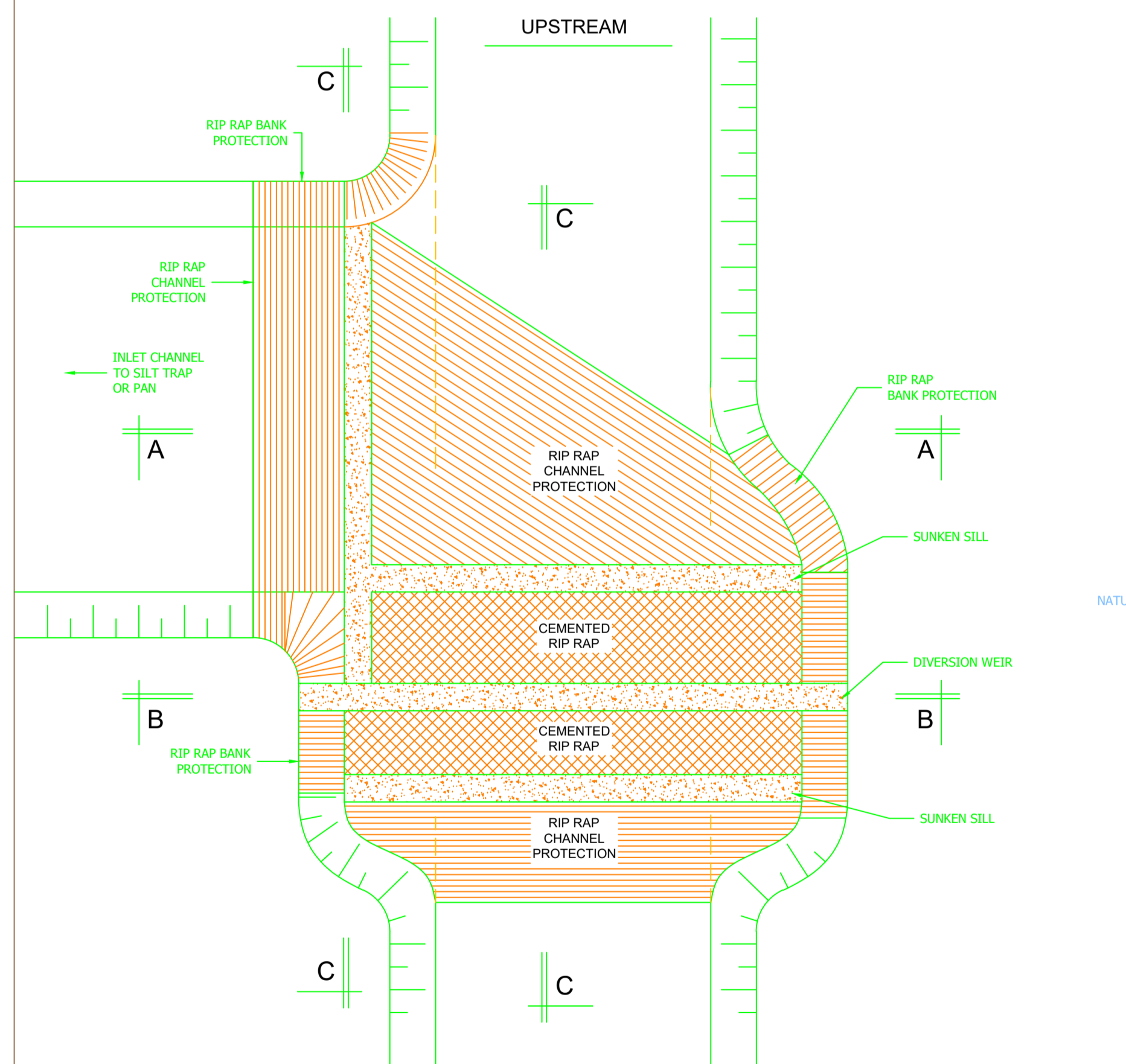
PLAN VIEW SCALE 1:50
