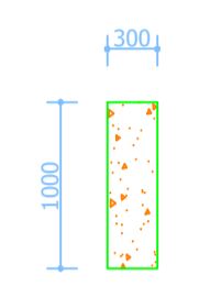
SECTION E-E SCALE 1:50
