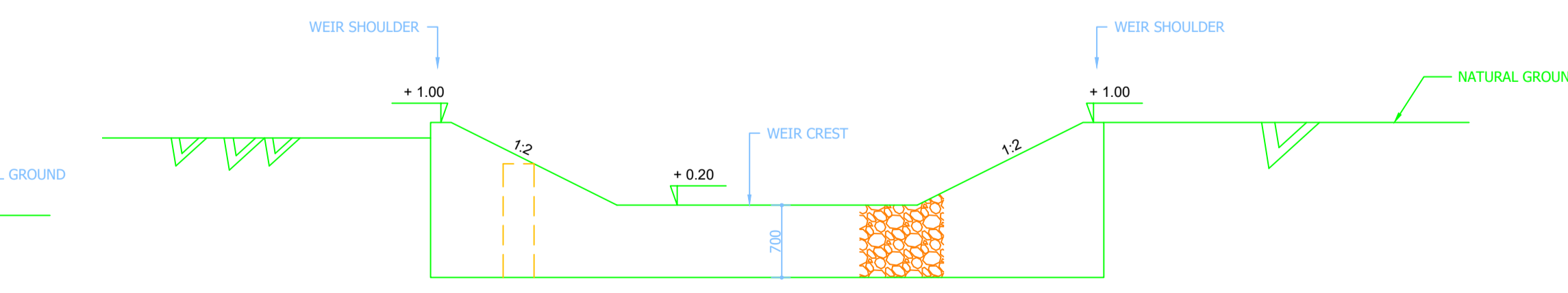
CROSS SECTION B-B SCALE 1:50
