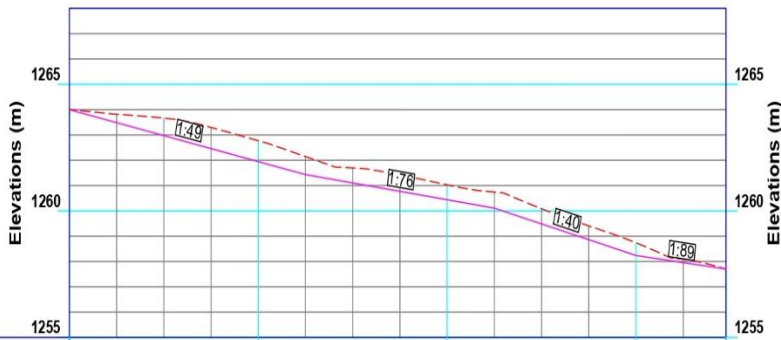
LONDUGOKWE DAM SPILLWAY PROFILE
