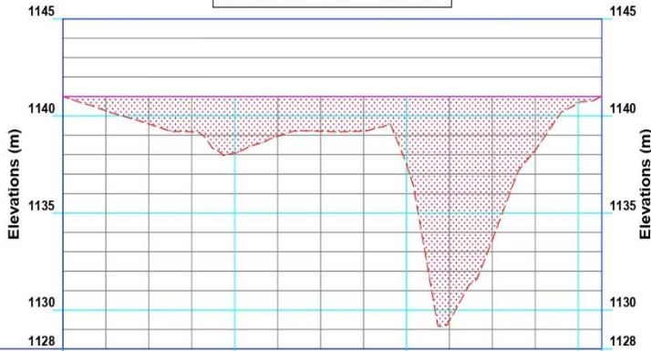
EMBANKMENT PROFILE
