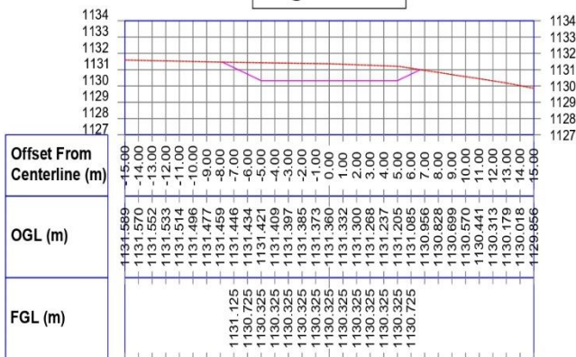
SPILLWAY SECTION @Km 0+250
