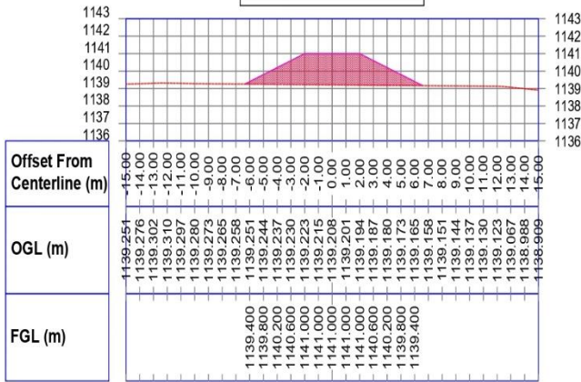
EMBANKMENT SECTION @Km 0+150
