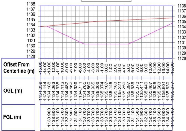
SPILLWAY SECTION @Km 0+225
