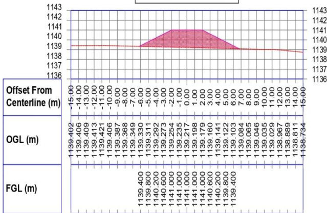
EMBANKMENT SECTION @Km 0+175
