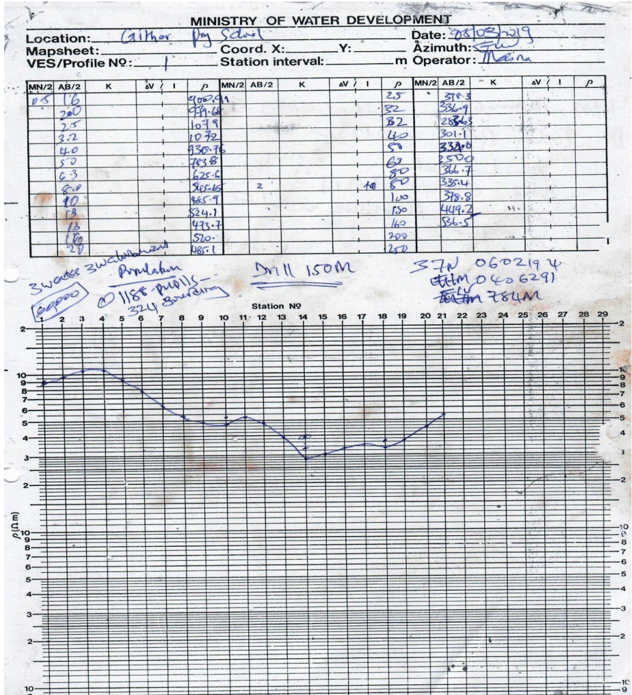
Fig 6.0: Resistivity curve for VES-1 at Gather Primary School
