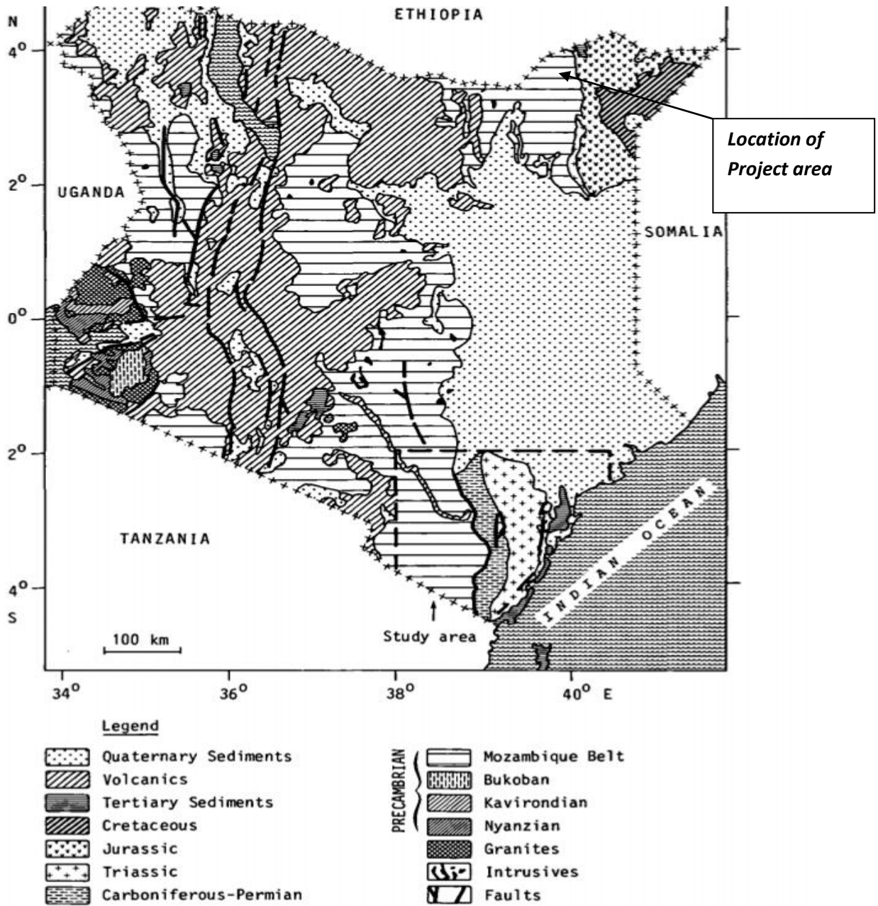
Fig. 2 Geology of Kenya (after Walsh, 1970)
