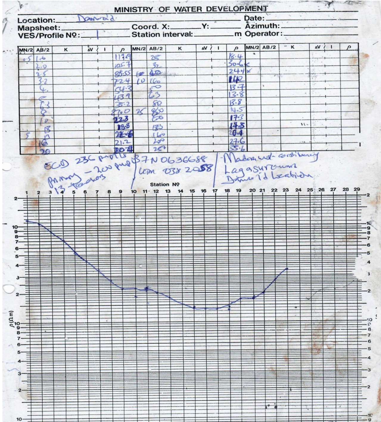
Fig 6.0: Resistivity curve for VES-1 at Darweid Primary School
