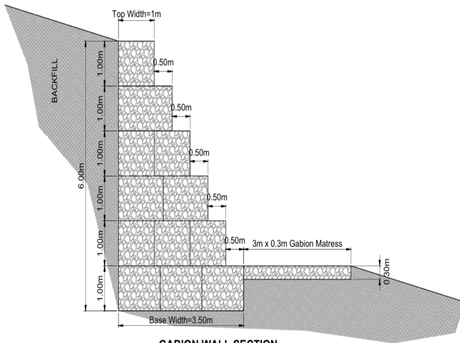
GABION WALL SECTION
