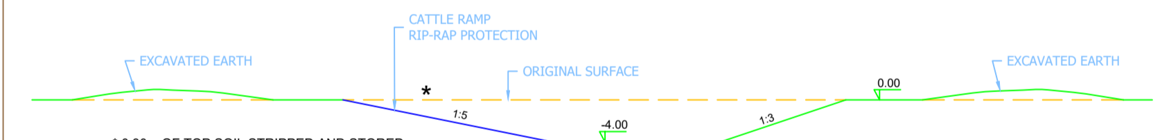
SECTION A-A SCALE 1:500
