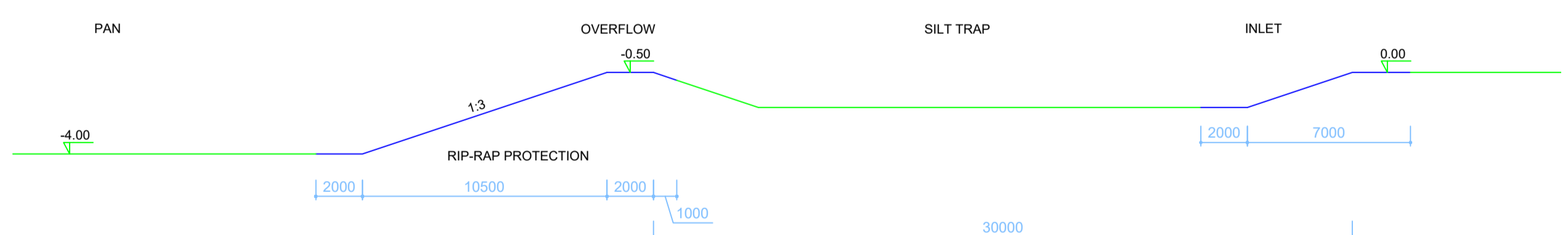
SILT TRAP DETAIL (B-B) SCALE 1:200
