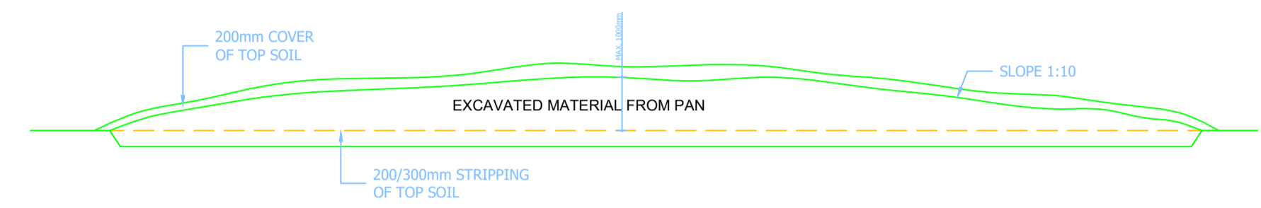
TYPICAL SECTION OF DISPOSED MATERIAL SCALE 1:100
