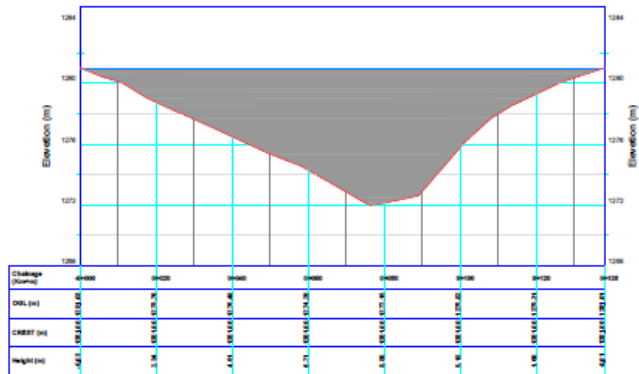
EMBANKMENT PROFILE
